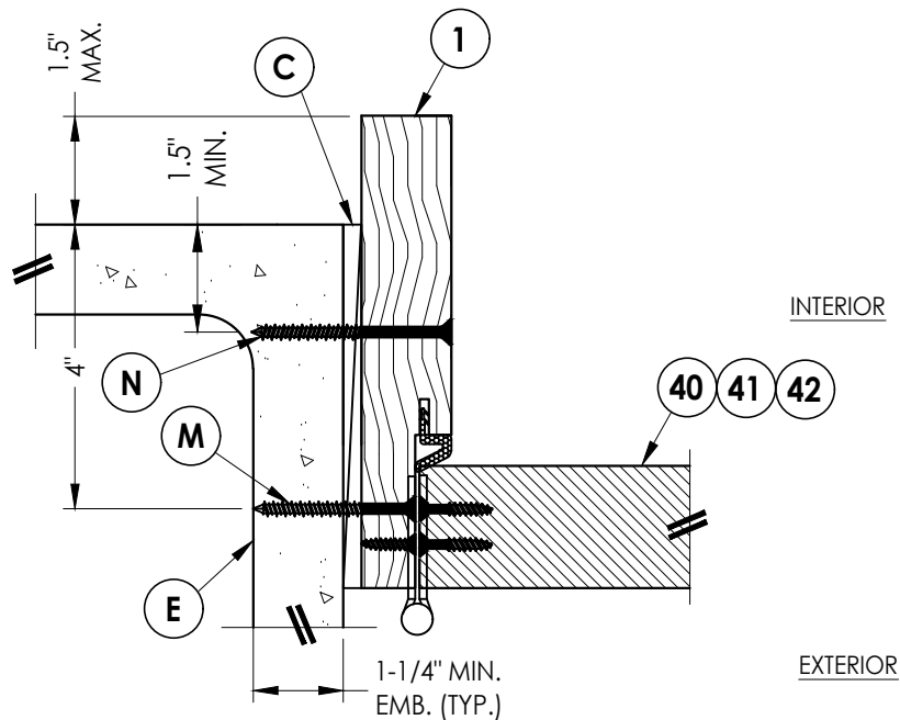
4 6 HORIZONTAL CROSS SECTION Shown Direct to Masonry Outswing only w/ 6-9/16" jamb
