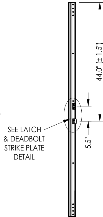
ASTRAGAL Latch & Deadbolt
