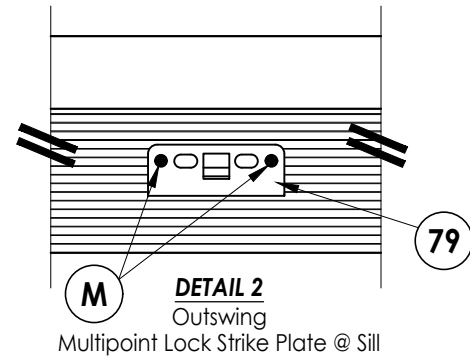
MULTIPOINT LOCK STRIKE DETAILS
