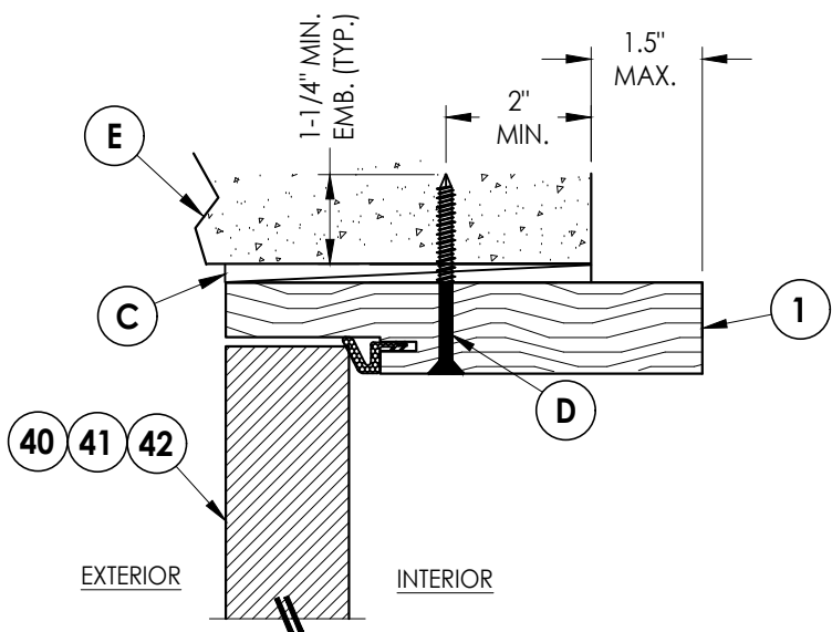
3 6 VERTICAL CROSS SECTION Shown Direct to Masonry Outswing only w/ 6-9/16" jamb
