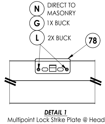
MULTIPOINT LATCH & DEADBOLT STRIKE PLATE DETAIL
