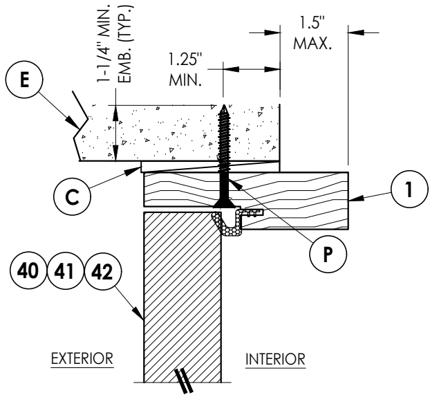
2 6 VERTICAL CROSS SECTION Shown Direct to Masonry Outswing only w/ 4-9/16" jamb Double Door Only (N/A w/ Sidelites)
